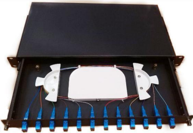
Fiber Patch Panel (Metal - 12 ports)
